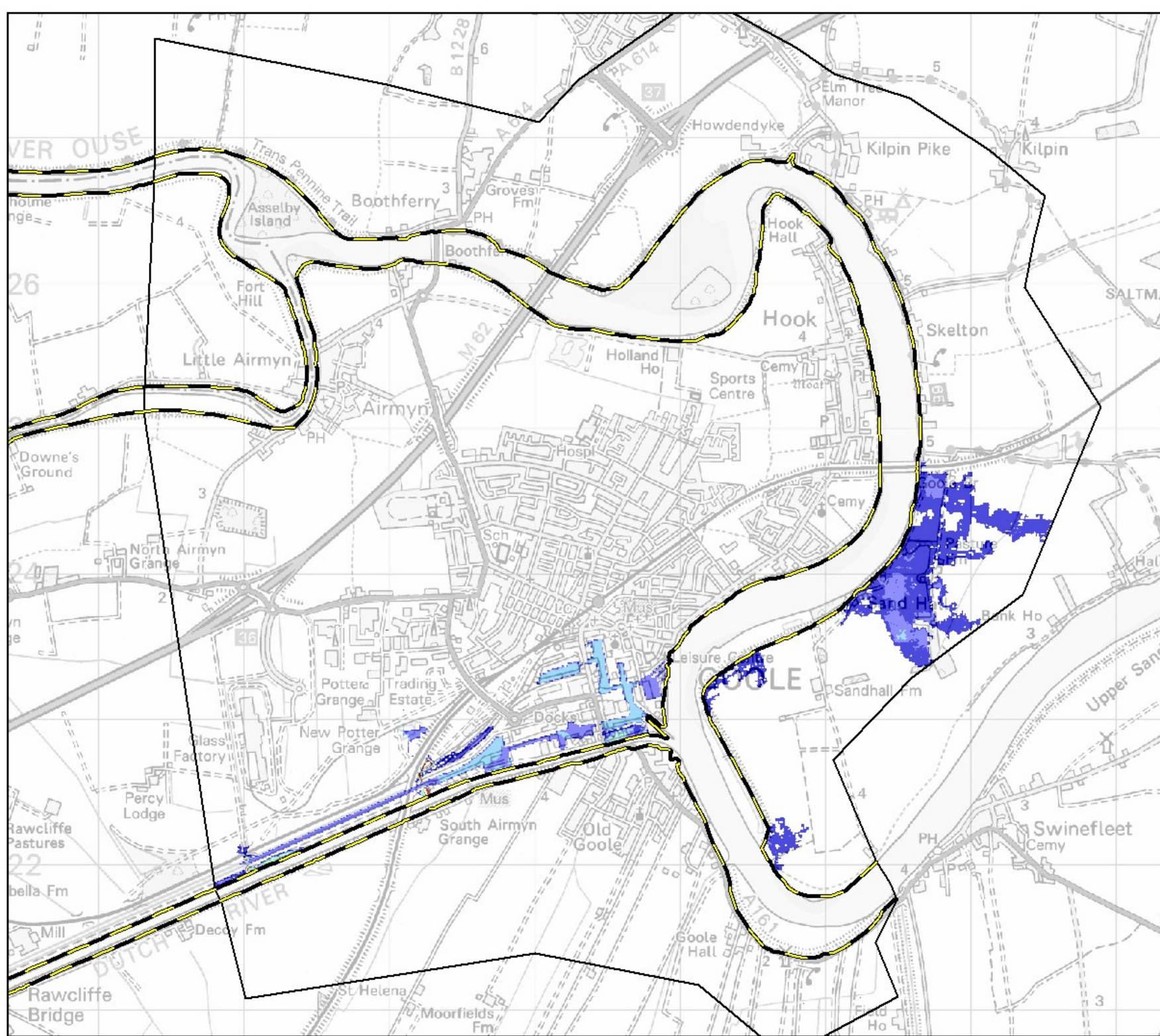
Figure A.1 Defence Overtopping 0.5% AEP (1 in 200 year)
