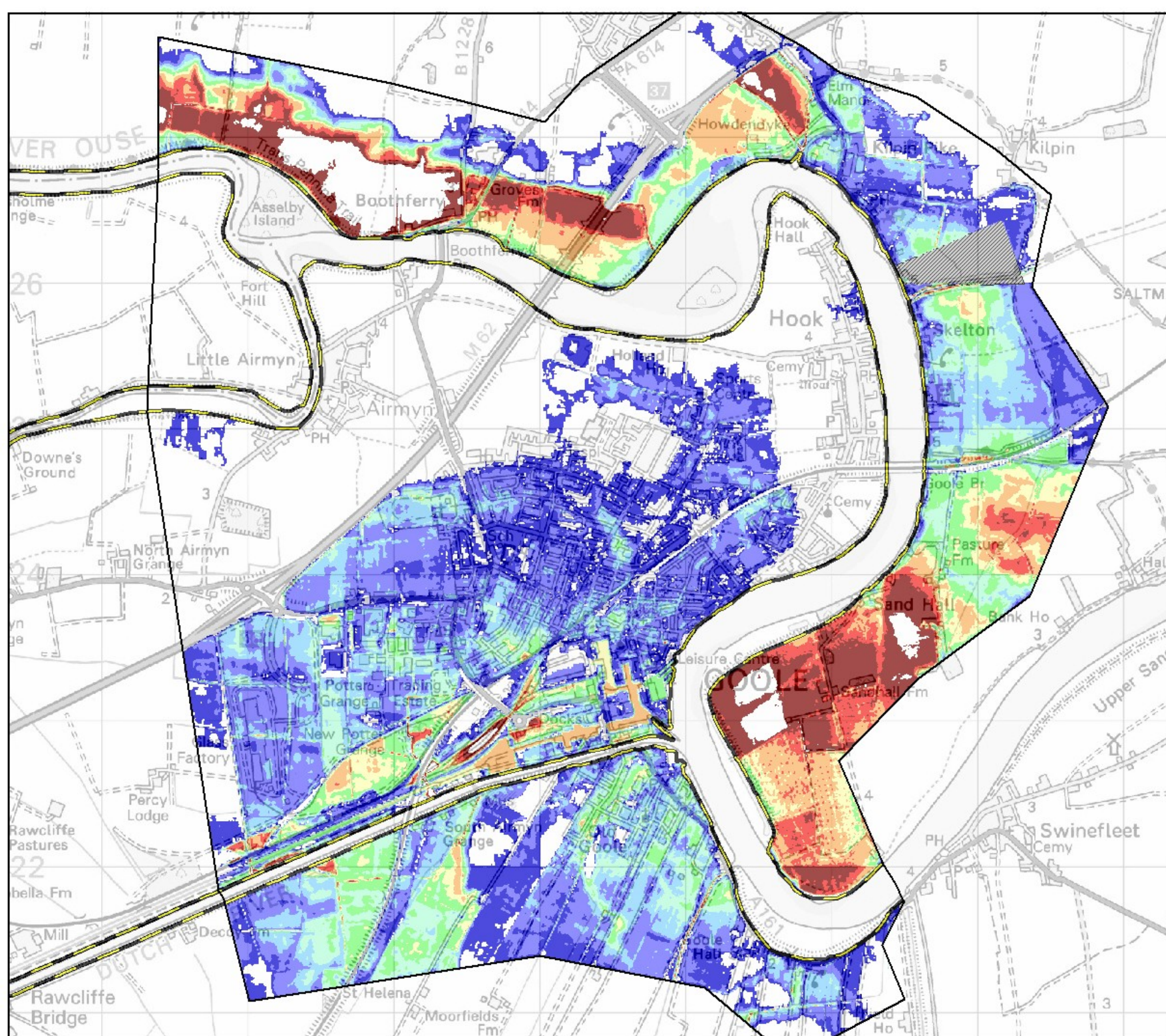
Figure B.1 Defence Overtopping 0.5% AEP (1 in 200 year) plus Climate Change
