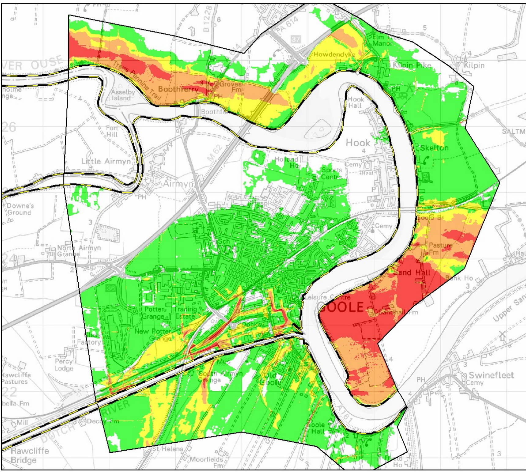
Figure B.2 Defence Overtopping 0.5% AEP (1 in 200 year) plus Climate Change
